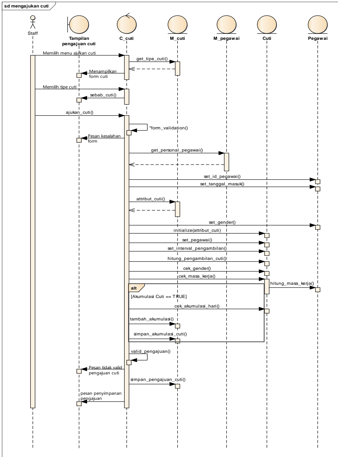
Lampiran 2. Sequence diagram Staff mengajukan cuti
