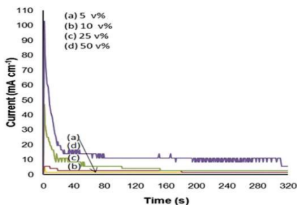
Fig. 2. The currents generated during anodization process at difference v% water content: (a) 5, (b) 10, (c) 25 and (d) 50.
