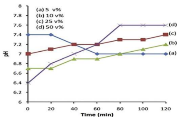
Fig. 3. The pH values during anodization process at difference v% water content: (a) 5, (b) 10, (c) 25 and (d) 50.
