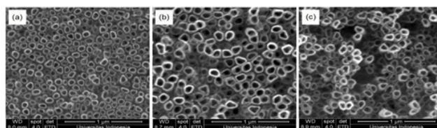
Figure 1. Top view FESEM image of (a) TNTA-U10, (b) TNTA-U30 and (c) TNTA-U60
