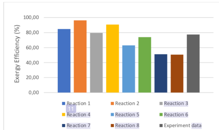
Figure 3. Exergy efficiency of syngas product at 723 K
