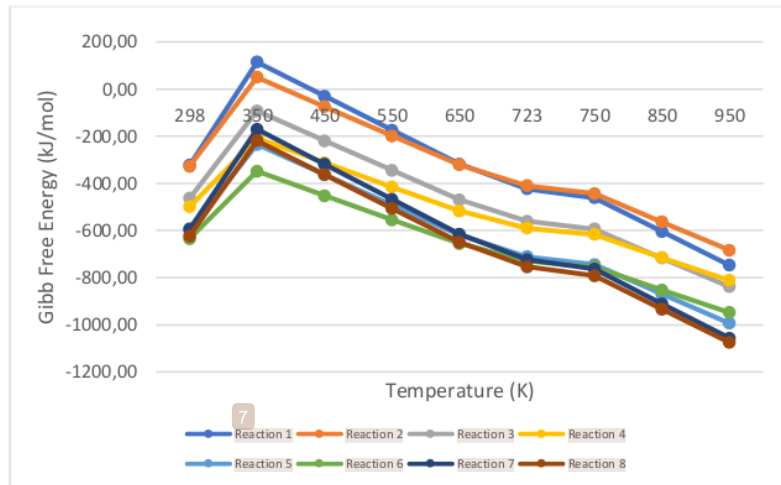
Figure 2. Gibbs free energy of cellulose pyrolysis
