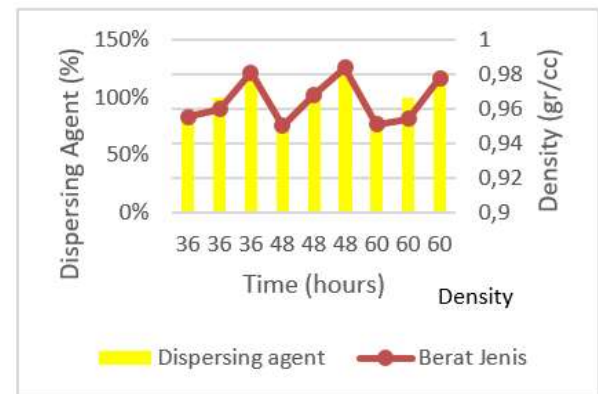
Figure 4. effect of milling time with different percentage of dispersing agent on density.
