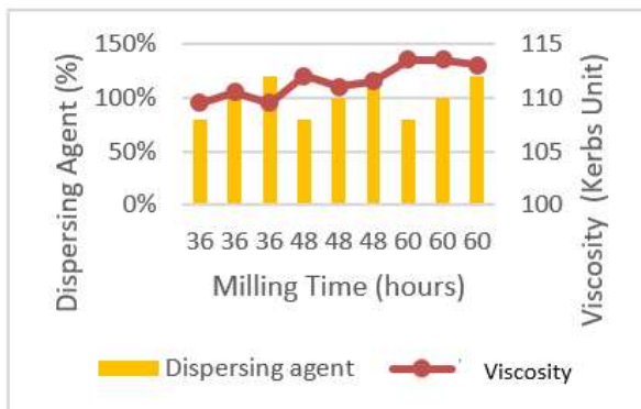
Figure 2. Effect of milling time with different percentage of dispersing agent on viscosity .
