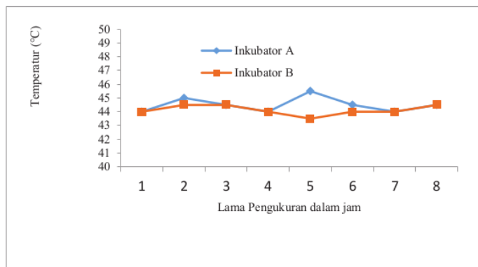
Gambar 4. Nilai temperatur inkubator skala 44
